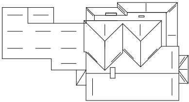
Elevation Roof Plan
