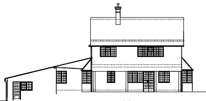
Front Elevation (Northside)
