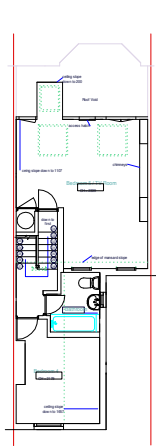
Second Floor
